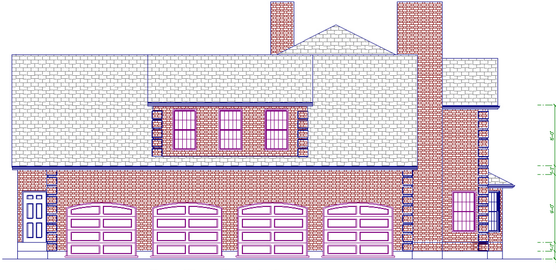
Left Side Elevation View
