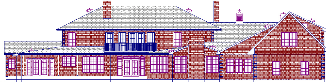
Rear Elevation View
